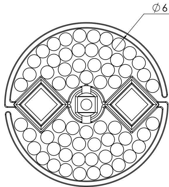
CAT 6 62 CABLES
