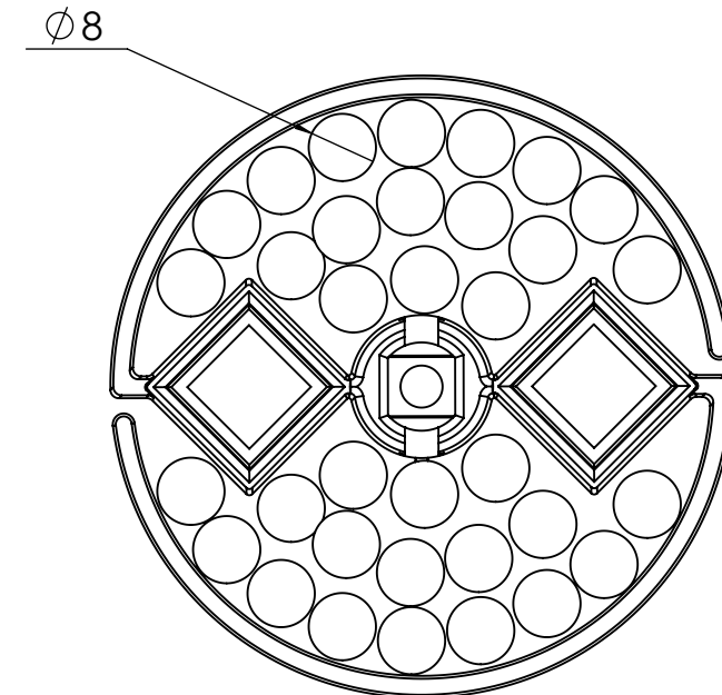
CAT 7 34 CABLES
