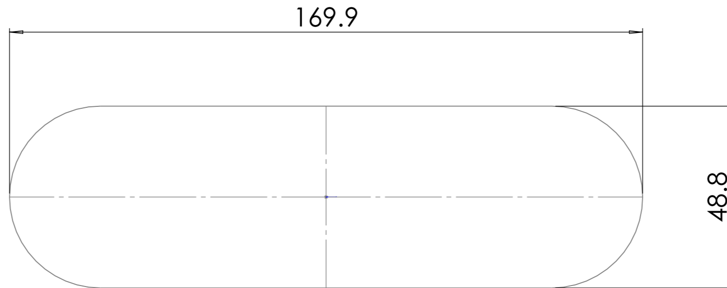
ROUTING CUTOUT 169.9mm X 48.8mm -0/+0.25mm
