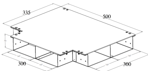
'T' fitting
