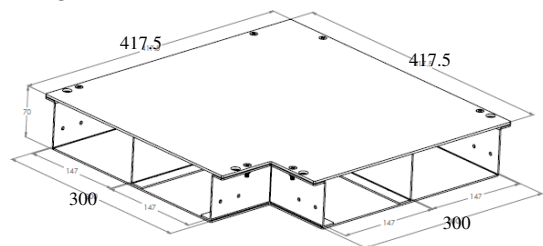
Bend fitting
