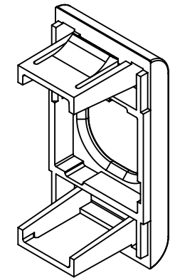
REAR ISOMETRIC
