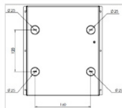
CONDUIT LOCATION 3 Base Box Standard 25mm knock-outs
