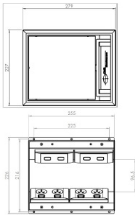
SECTION THRU-BOX
