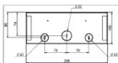
CONDUIT LOCATION 1 Outlet Sides Enlarged 32mm knock-out for easier passthrough
