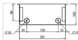
CONDUIT LOCATION Hinge & Exit Sides Standard 25mm knock-out
