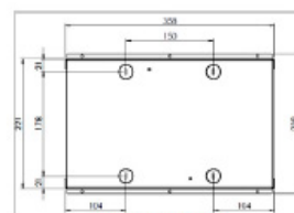
CONDUIT LOCATION Base Box Standard 25mm knock-outs
