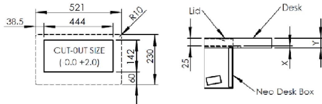
SECTION
