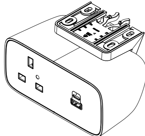
Z = UNDER DESK CLAMP
