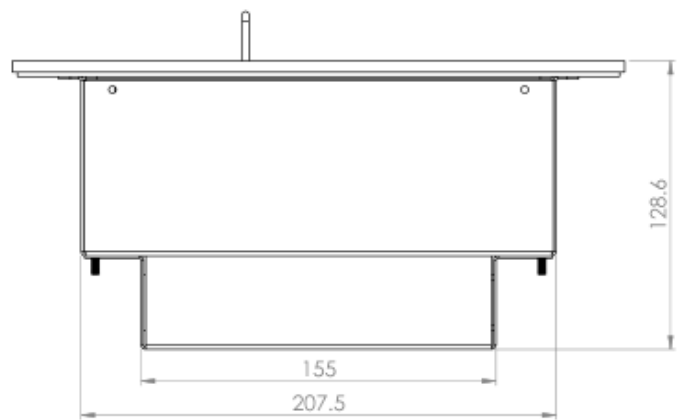
END VIEW
