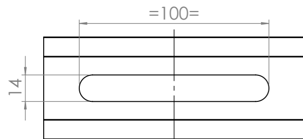
ZEUS DATA EXIT CUTOUT TO SUIT 2 X DATA
